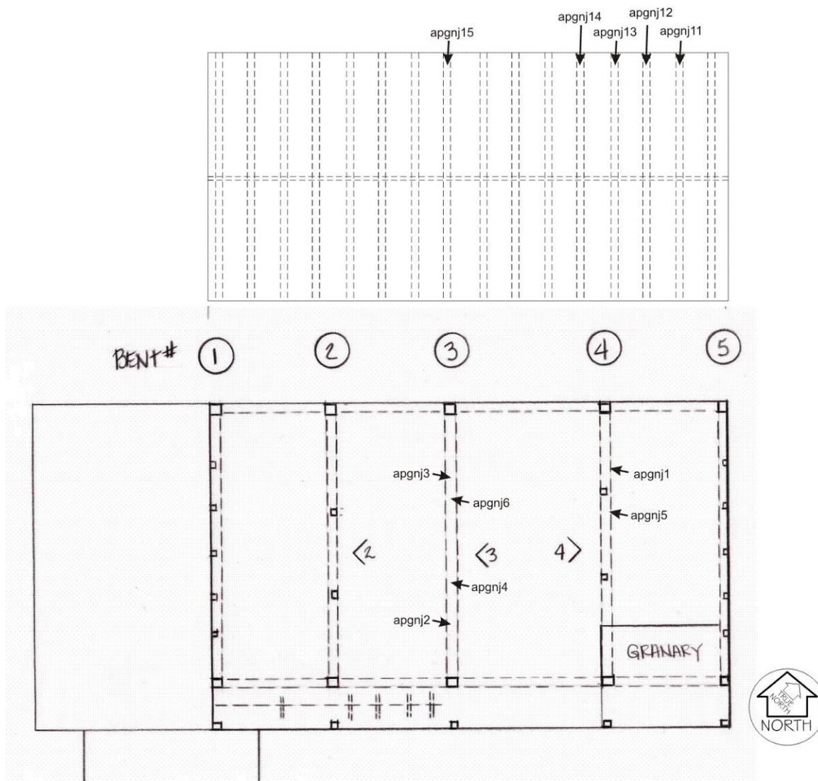
Figure 4. Modified drawing of the Apgar Barn showing sample locations from the 1 st floor (top) and 2 nd floor (bottom) (after Cielo 2014)
