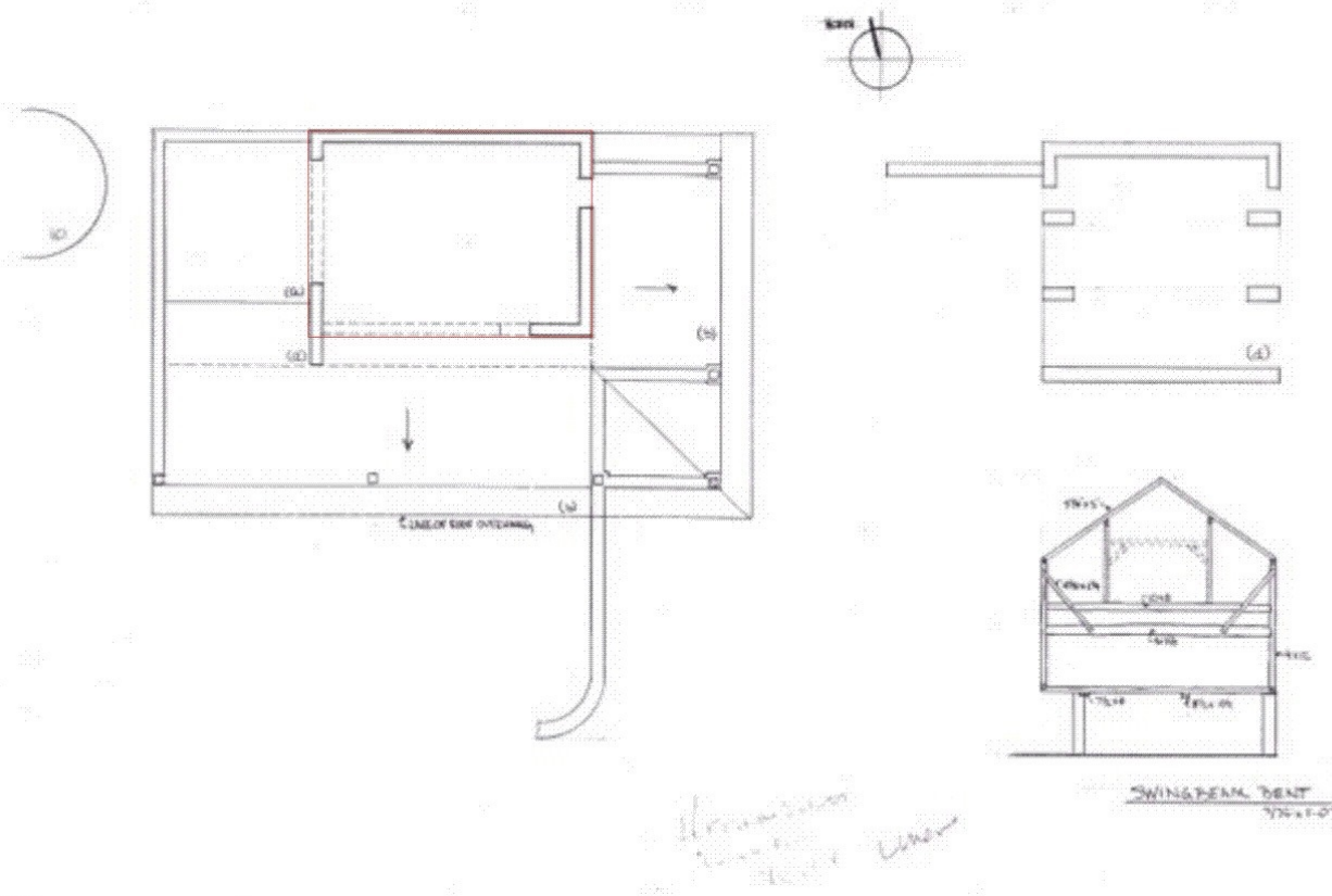
Figure 2. Drawing of Blair Barn site by Carla Cielo, with a red square around the original barn.
