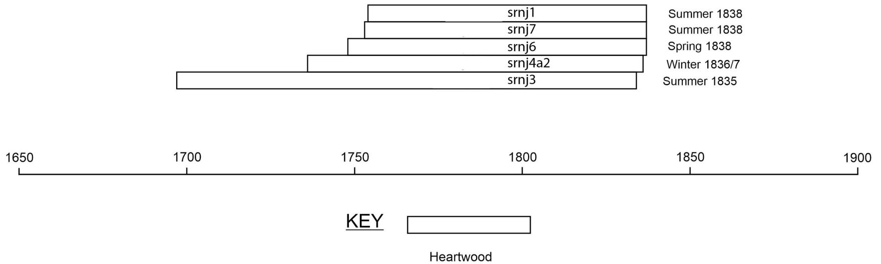
Figure 4. Bar diagram showing dated timbers in chronological order.
